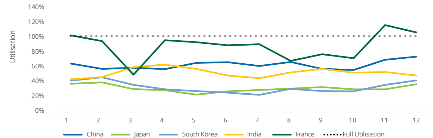
Figure 7.4: Monthly regasification utilisation by top five LNG importers, 2023
