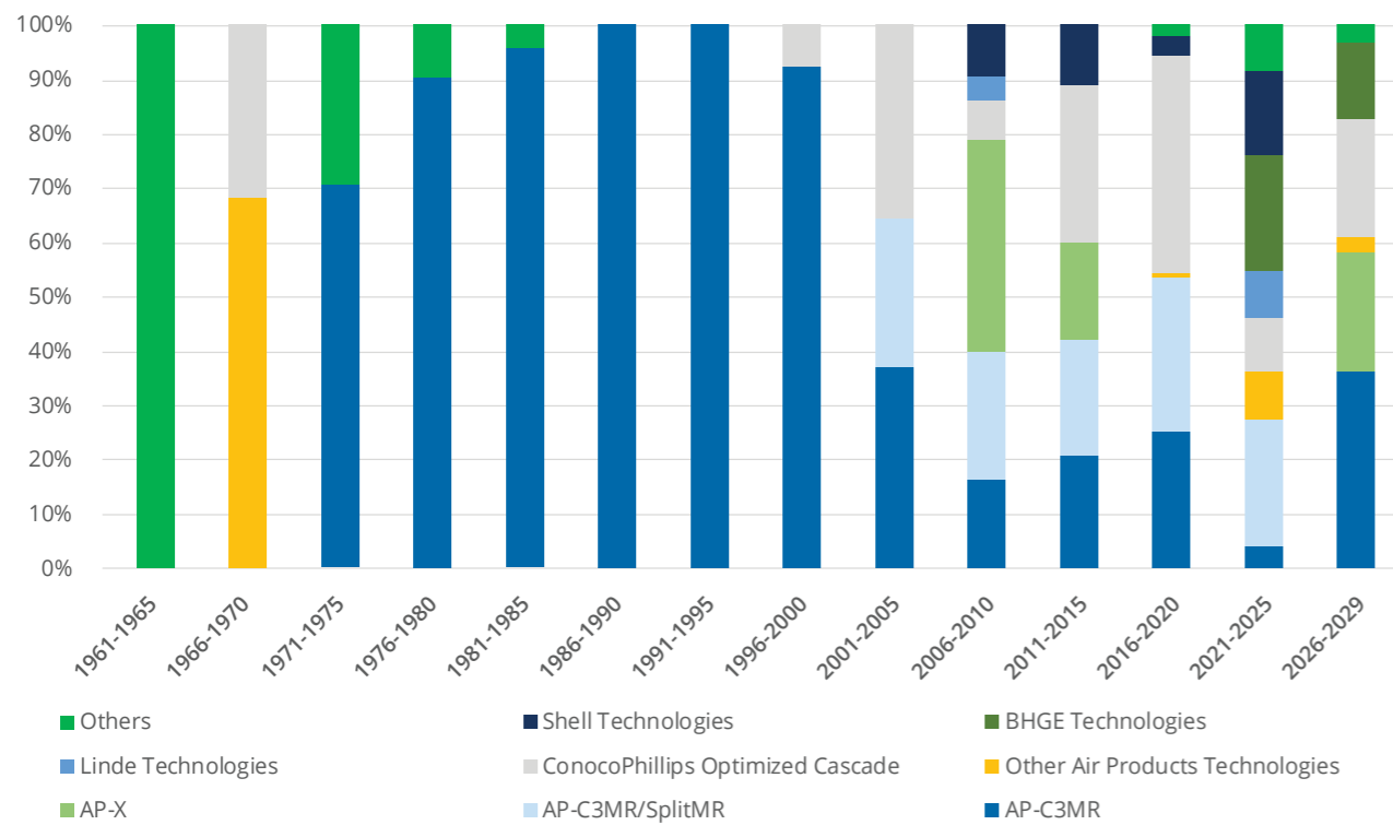
Figure 5.9: Share of installed and future approved liquefaction capacity by technology and start-up year, 1961-2029
